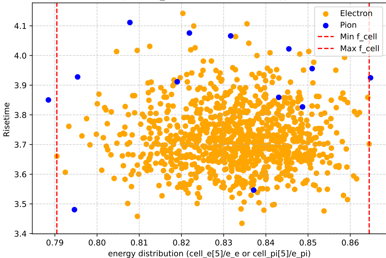
Scatter plot of f_cell vs risetime for energy 20.0GeV
